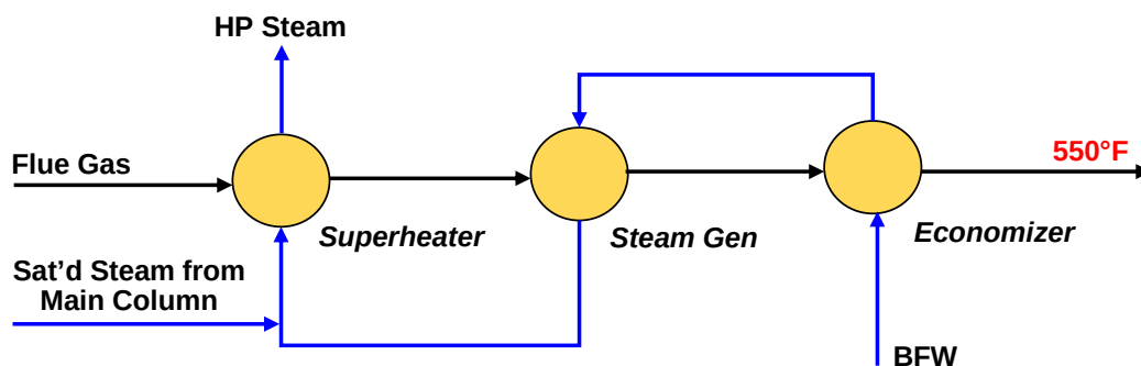
Figure 11 Conventional Flue Gas Cooler
