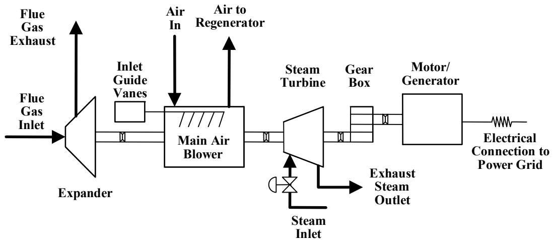
FIGURE 1 Traditional 5-Body Power Recovery Train
