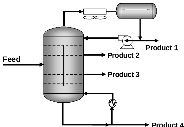
Figure 10 Gasoline Splitting Using a DWC with Two Side-Draws.
