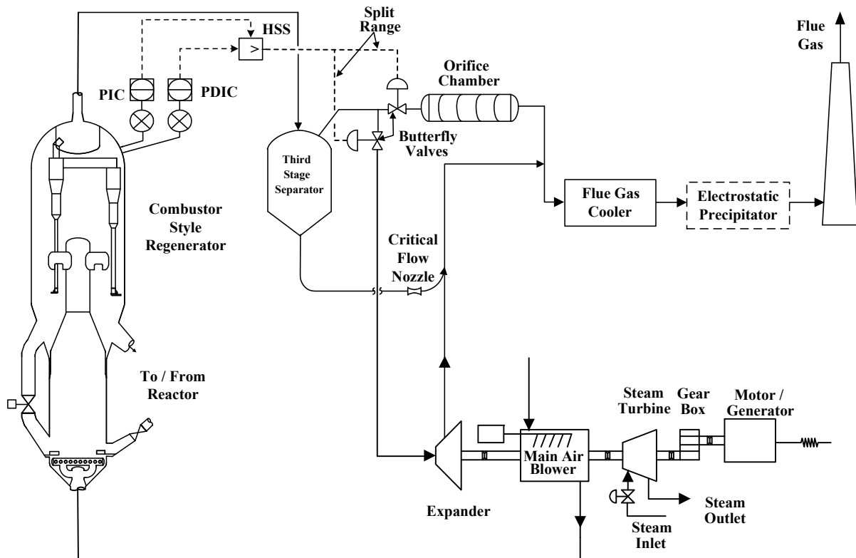
FIGURE 2 Traditional Power Recovery System – “Five-Body Train”
