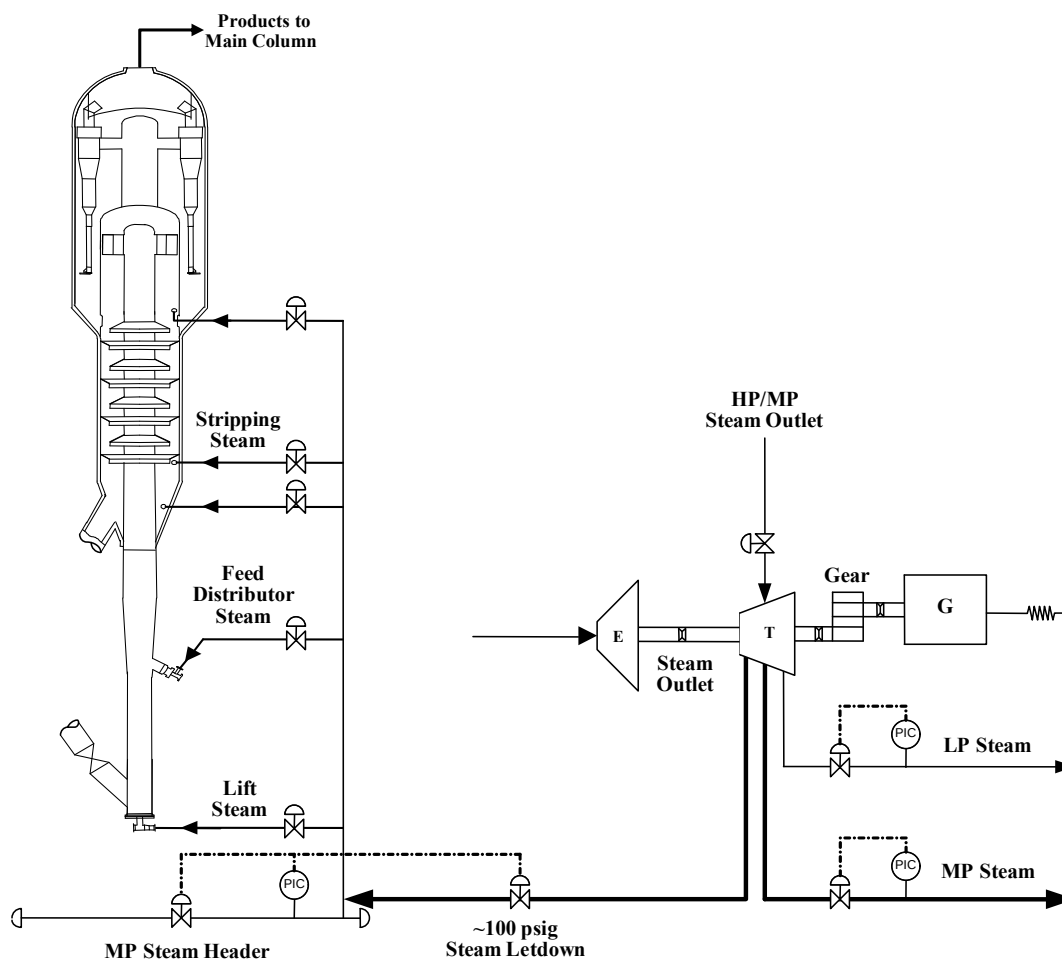
FIGURE 4 UOP Process Integrated Steam Turbine
