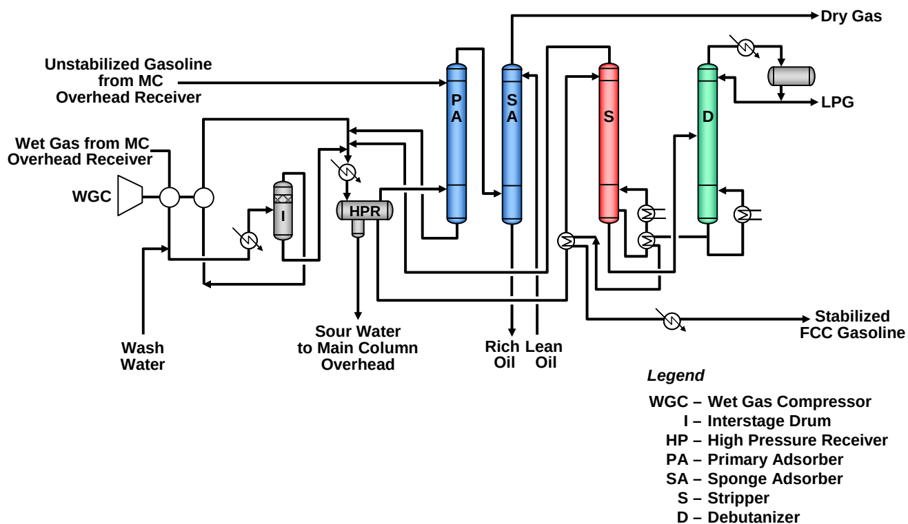
Figure 6 Typical Gas Concentration Unit
