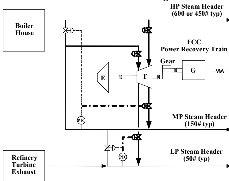
FIGURE 3 UOP Steam Letdown Configuration
