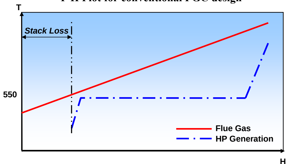
Figure 12 T-H Plot for conventional FGC design
