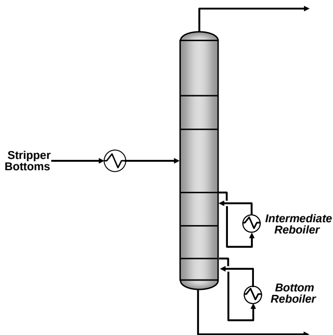
Figure 7 Proposed Debutanizer Reboiler Configuration
