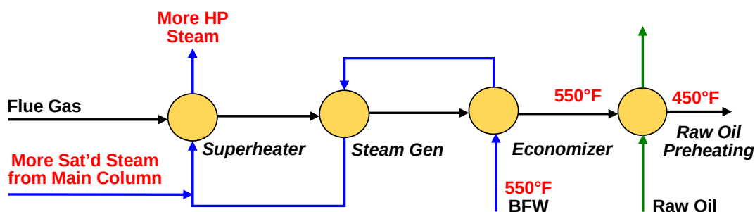
Figure 13 Novel Flue Gas Cooler
