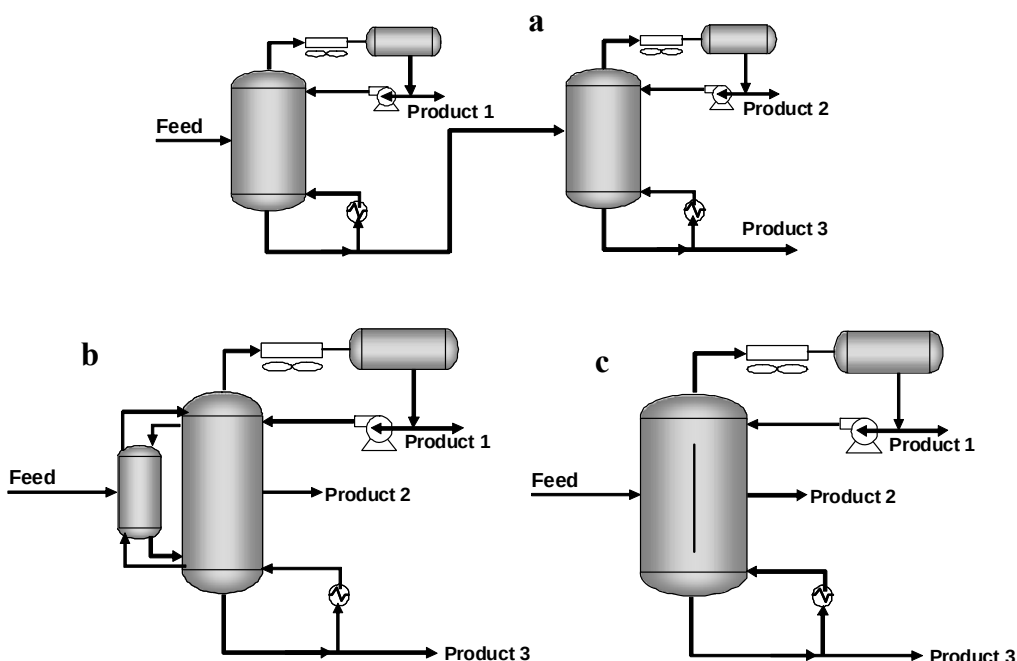
Figure 8 Conventional Distillation Sequence (a), Petlyuk Column (b) and DWC (c).
