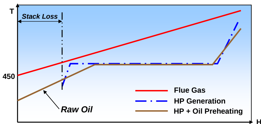
Figure 14 T-H Plot for Novel Flue Gas Cooler
