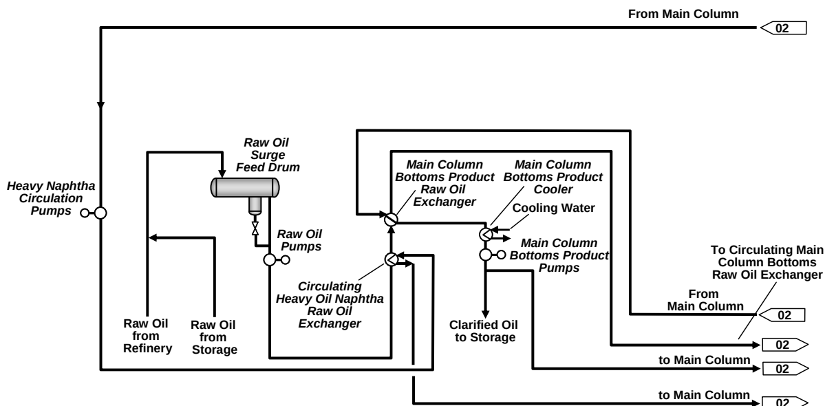
Figure 5 Non-Direct Feed Configuration
