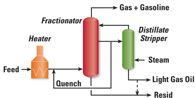
Figure 1 ■ Typical Visbreaking Process
