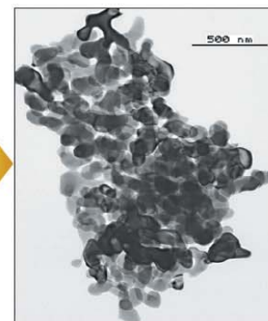
Versal Alpha Alumina (8 m 2 /g) Derived from Pseudoboehmite
