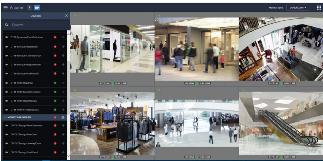
Device tree
